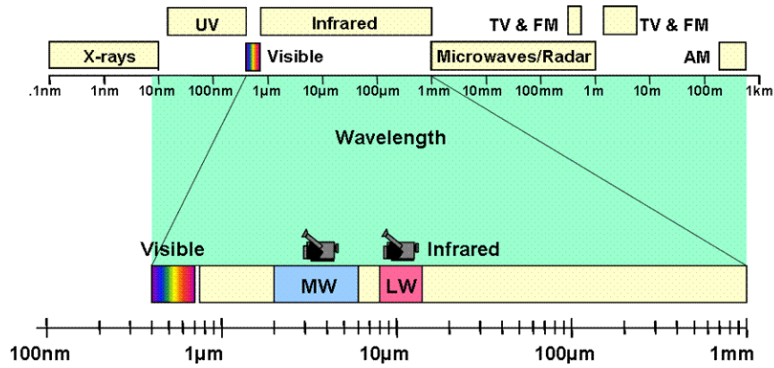
Figure 8-5: Electromagnetic Spectrum
